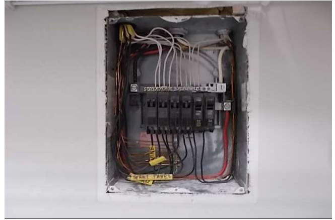
Panel interior
